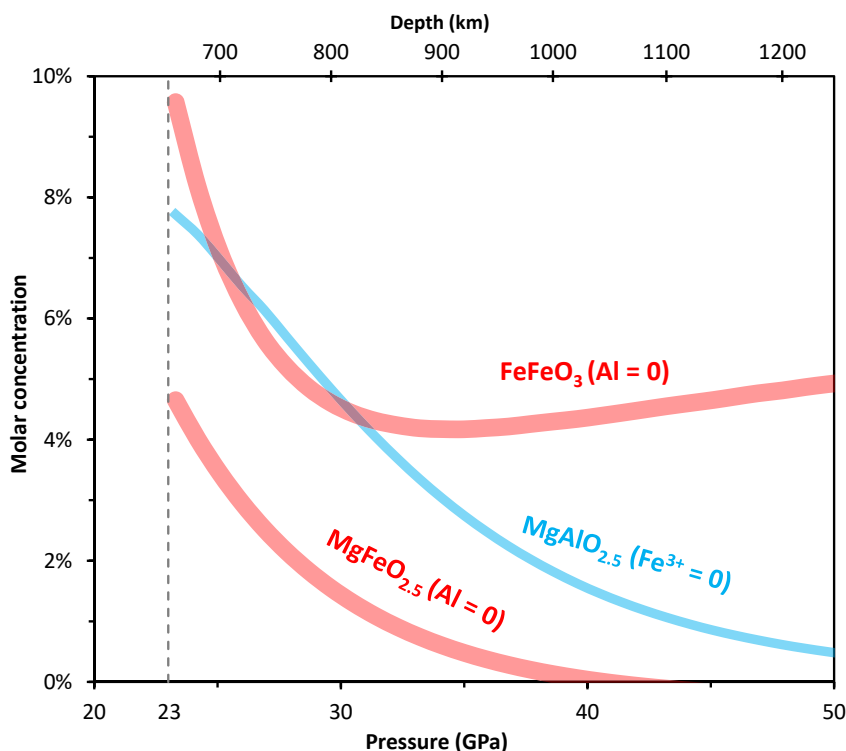
Figure 10. \text{FeFeO}_3 and \text{MgFeO}_{2.5} contents as a function of depth according to the pressure dependences determined in this study, temperature dependences given by Fei et al. (2020), and geotherm from Katsura et al. (2010). The \text{MgAlO}_{2.5} content in \text{Fe}^{3+} -free bridgmanite is based on the pressure and temperature dependences given by Liu, Ishii, and Katsura (2017) and Liu, Akaogi, & Katsura (2019).
