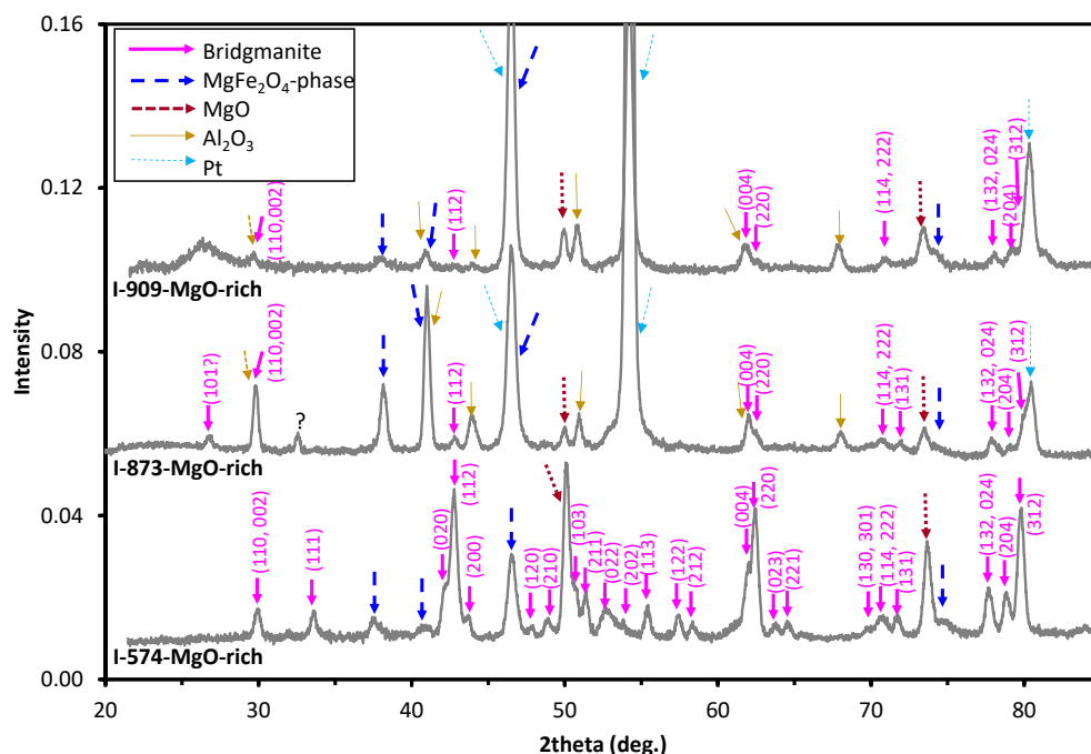
Figure 4. X-ray diffraction spectra of the recovered samples (MgO-rich conditions). Pt and \text{Al}_2\text{O}_3 peaks are from the sample capsule and the sleeve outside of the capsule in the cell assembly (Figure 2), respectively, owing to the limited spatial resolution of the diffractometer. The \text{MgFe}_2\text{O}_4 -phase show consistent peaks at different pressures, indicating the same structure. The spectra are background subtracted. The identified peaks of bridgmanite are labeled in the figure (hkl), and their d-spacings and fitted lattice parameters are given in the online Supporting Information (Table S1).
