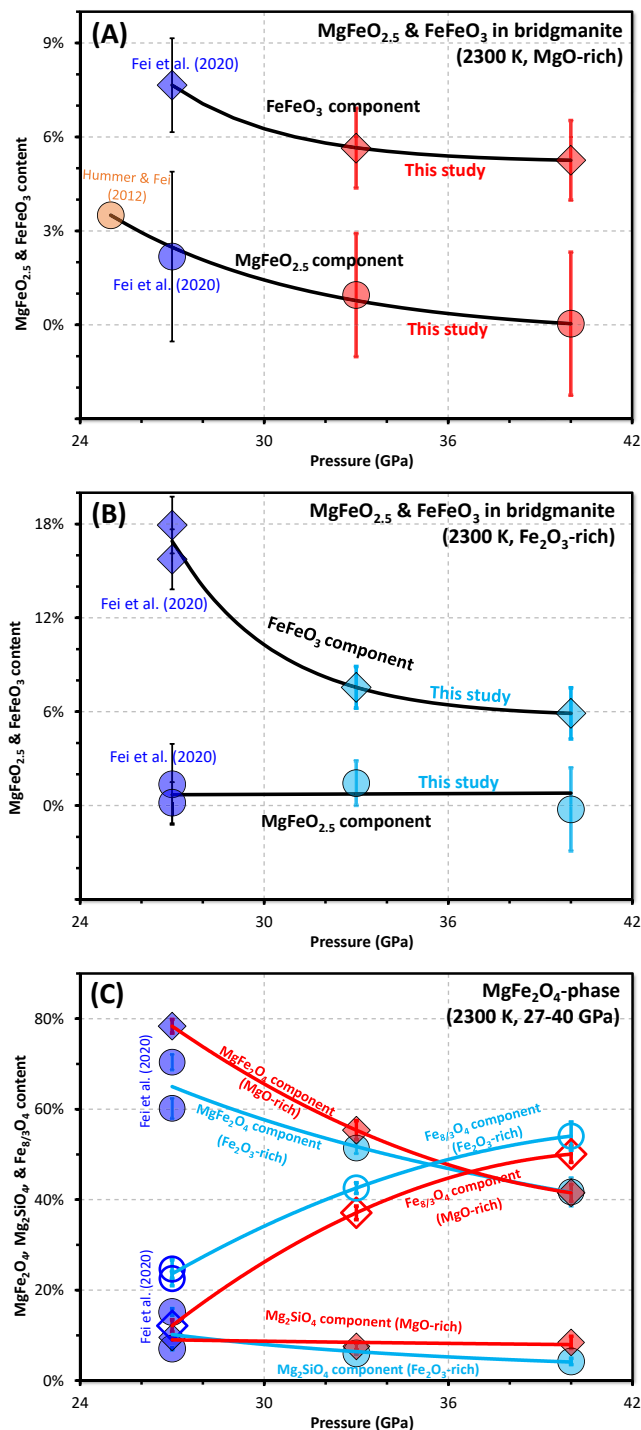
Figure 8. Substitution mechanisms in bridgmanite and \text{MgFe}_2\text{O}_4 -phase. (a) \text{Fe}^{3+} substitution in bridgmanite under MgO-rich conditions. The maximum \text{MgFeO}_{2.5} content reported by Hummer and Fei (2012) at 25 GPa, 1,970–2,070 K is also shown for comparison. (b) \text{Fe}^{3+} substitution in bridgmanite under \text{Fe}_2\text{O}_3 -rich conditions. (c). Substitution mechanisms in the \text{MgFe}_2\text{O}_4 -phase. The data points with blue symbols at 27 GPa are from Fei et al. (2020). The error bars represent one standard deviation of the analyzed points by electron microprobe as shown in Table 1.
