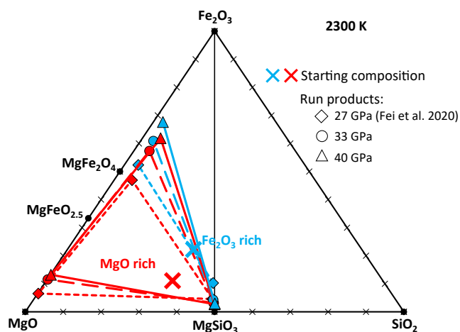
Figure 1. Chemical compositions of MgO-rich and Fe 2 O 3 -rich starting materials and run products in the ternary phase diagram with endmembers of Fe 2 O 3 , MgO, and SiO 2 . The 27 GPa run was already reported in Fei et al. (2020).
