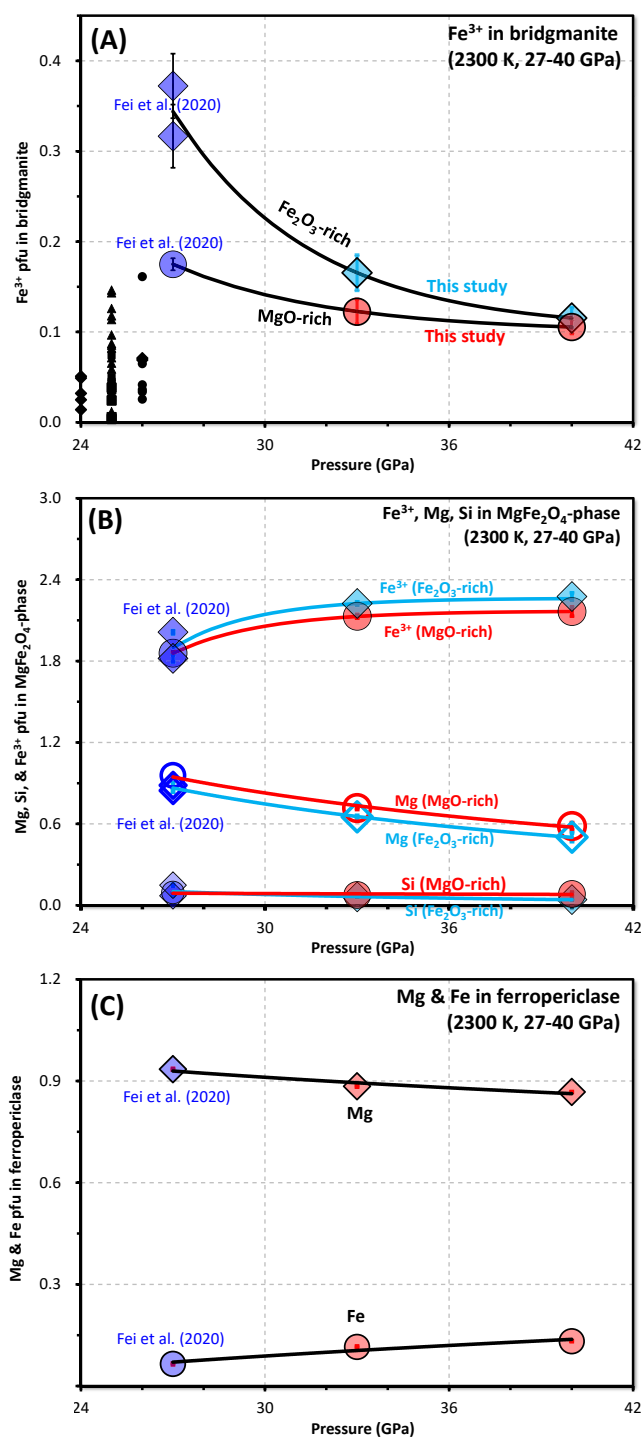
Figure 7. Chemical composition of bridgmanite, ferropericlasite, and \text{MgFe}_2\text{O}_4 -phase in run products. (a) \text{Fe}^{3+} content in bridgmanite calculated to O = 3. (b) Mg, Si, and \text{Fe}^{3+} contents in the \text{MgFe}_2\text{O}_4 -phase calculated to O = 4. (c) Mg and Fe content in ferropericlasite from MgO-rich samples calculated to O = 1 assuming that all Fe is ferrous in ferropericlasite. Black symbols represent the \text{Fe}^{3+} content in bridgmanite that coexists with ferropericlasite reported in previous studies (Frost & Langenhorst, 2002; Frost et al., 2004; Huang, Boffa-Ballaran, McCammon, Miyajima, Dolejš & Frost, 2021; Hummer & Fei, 2012; Lauterbach et al., 2000), all of which are lower than this study because their experimental temperatures are lower, and/or \text{MgFe}_2\text{O}_4 -phase did not appear (namely \text{Fe}^{3+} is not saturated). The data points with blue symbols at 27 GPa are from Fei et al. (2020). The error bars represent one standard deviation of the analyzed points by electron microprobe as shown in Table 1.
