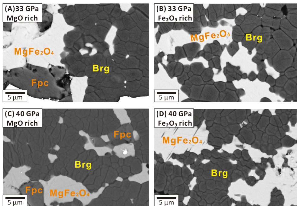
Figure 3. SEM images of samples recovered from 33 (a, b) and 40 GPa (c, d). Brg: bridgmanite. Fpc: ferropericlaase. \text{MgFe}_2\text{O}_4 : \text{MgFe}_2\text{O}_4 -phase.
