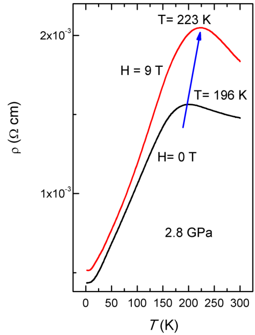
FIG. 4. Temperature dependence of the resistivity in magnetic fields H = 9 T and H = 0 T at 2.8 GPa. The curves are a guide to the eye.
