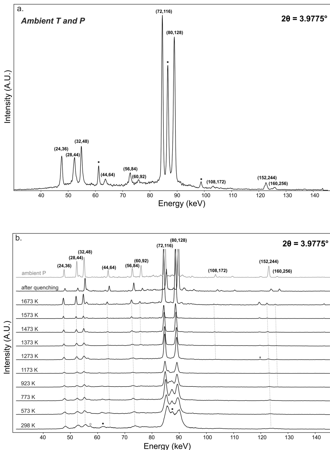
Figure 1 | (a) XRD pattern in energy-dispersive mode of i-QC starting material at ambient conditions. Filled circles indicate peaks representative of a secondary phase (AlFe 3 ) resulting from the synthesis procedure. (b) Temperature dependence of XRD patterns for i-QC. Notes: (*) MgO from surrounding sleeve; (•) AlFe 3 ; (°) graphite peak from the surrounding capsule.
