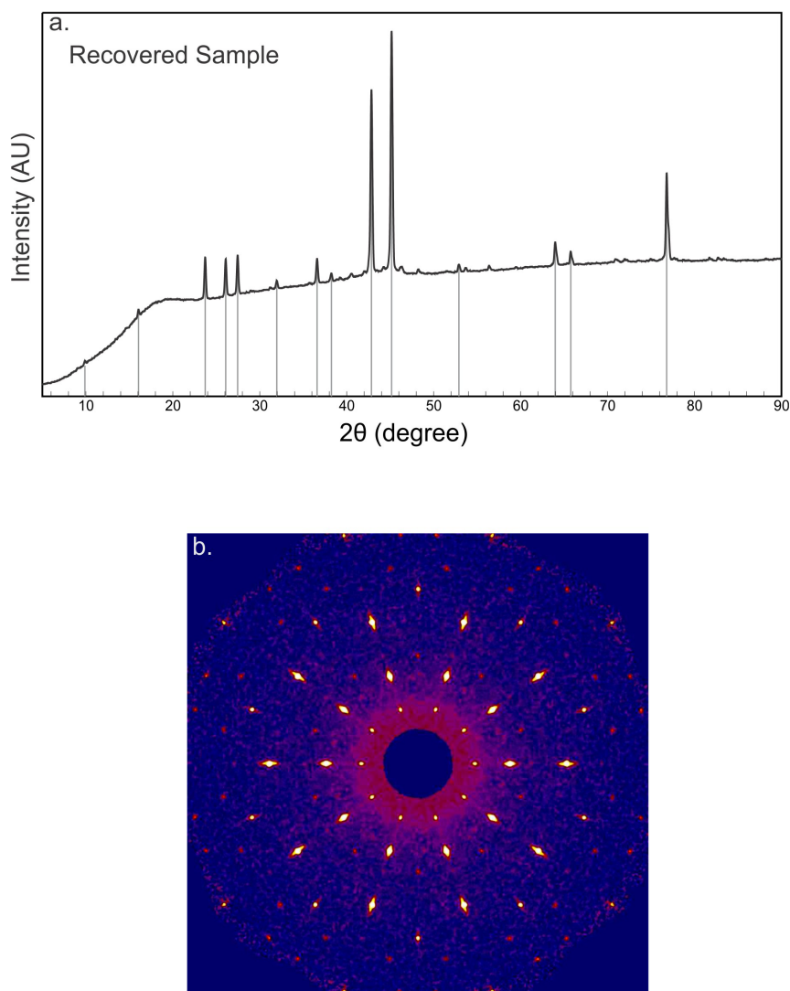
Figure 7 | X-ray powder diffraction pattern (CuK \alpha radiation) of the sample recovered from 5 GPa and 1673 K (a). Grey lines are used to mark peaks representative of i-AlCuFe that can be indexed according to Bindi et al. 6 (see also Figure S1b). b) A reconstructed precession image down the five-fold symmetry axis obtained using the collected single-crystal X-ray reflections from a fragment of the same sample as in (a) compatible with icosahedral symmetry.
