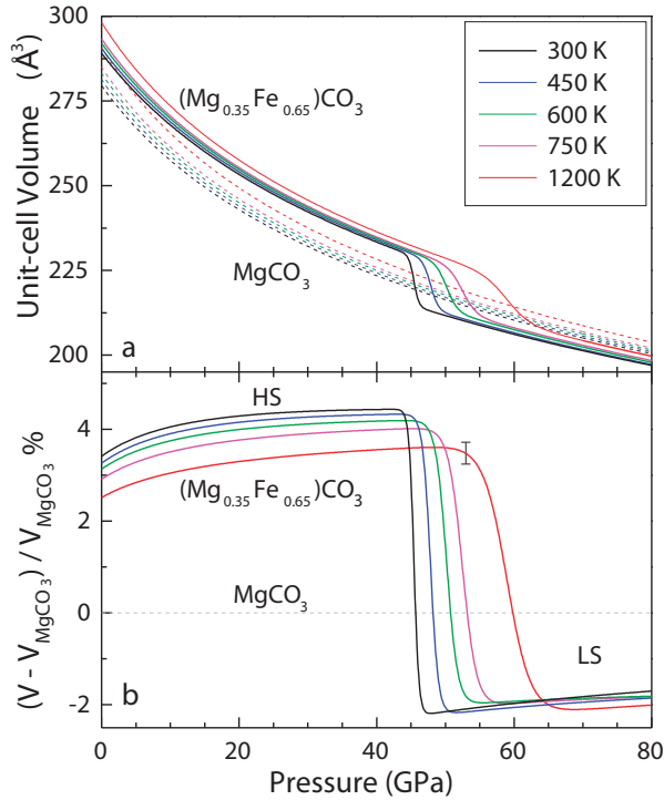
FIGURE 10. Comparison of the thermal pressure-volume relations (a) and volume differences (b) between magnesiosiderite and magnesite [MgCO 3 ] at high P - T . Solid lines in a: the fitted thermal P - V curves of magnesiosiderite; dashed lines: the fitted thermal P - V curves of magnesite (Zhang et al. 1997; Litasov et al. 2008). Solid lines in b show the volume differences across the spin transition using magnesite ( V_{\text{MgCO}_3} ) as the reference. Vertical ticks: representative errors. (Online color.)
