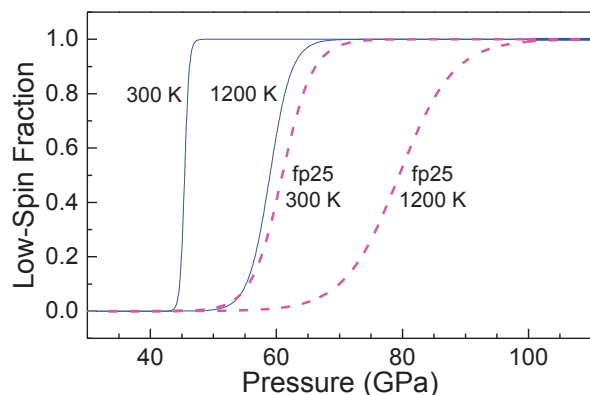
FIGURE 8. Comparison of the low-spin fraction between magnesiosiderite and ferropericlasite at high P - T . Solid lines = magnesiosiderite; dashed lines = ferropericlasite [(Mg 0.75 Fe 0.25 )O; fp25] (Mao et al. 2011). (Online color.)
