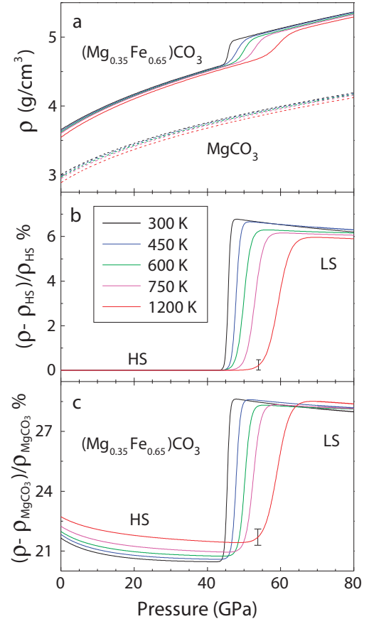
FIGURE 11. Comparison of the thermal pressure-density relations and density differences between magnesiosiderite and magnesite [MgCO 3 ] at high P - T . Solid lines in a: fitted thermal P - \rho curves of magnesiosiderite; dashed lines: fitted thermal P - \rho curves of magnesite (Zhang et al. 1997; Litasov et al. 2008). Solid lines in b show the density differences across the spin transition using the HS magnesiosiderite as the reference; Solid lines in c show the density differences across the spin transition using magnesite ( \rho_{\text{MgCO}_3} ) as the reference. Vertical ticks: representative errors. (Online color.)
