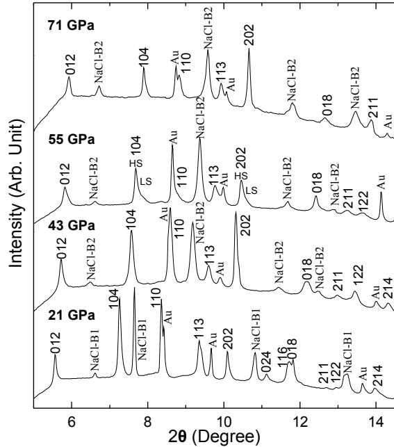
FIGURE 2. Representative X-ray diffraction patterns of magnesiosiderite [(\text{Mg}_{0.35}\text{Fe}_{0.65})\text{CO}_3] at high pressures and 1200 K measured from a LHDAC. HS and LS states are labeled to illustrate the splitting of the diffraction peaks across the spin transition. Gold (Au) was used as the internal pressure calibrant (Fei et al. 2007a), while sodium chloride (NaCl) in B1 or B2 structure was used as the thermal insulator and pressure medium. The wavelength of the monochromatic X-ray beam was 0.3344 Å.
