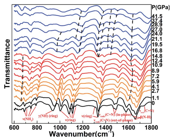
Fig. 4 IR spectroscopy of DAT as a function of pressure up to ~40 GPa. The black, orange, red and blue lines stand for the phase I to phase IV. The dash lines mark the new modes and their evolution. And other marks of the vibrational modes are same to the Raman spectra in Fig. 3.
