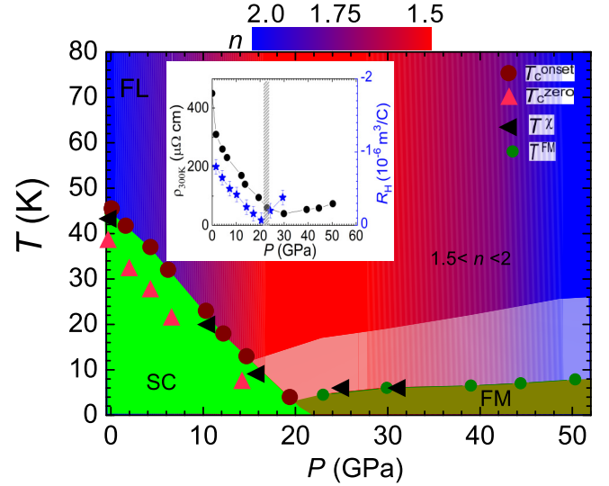
FIG. 3. Pressure-temperature ( P - T ) phase diagram of NdFeAsO 0.9 F 0.1 . Pressure dependence of the SC transition temperatures T_c s and a contour color plot of the normal-state resistivity exponent n up to 50 GPa. The temperature dependence of n are extracted from \rho(T) = \rho_0 + AT^n for each pressure. The pink region illustrates that the temperature dependence of n between 1.5 \leq n \leq 1.75 . The values of T_c^{\text{onset}} , T_c^{\text{zero}} , T_c^{\text{FM}} , and T_c^x were determined from the high-pressure resistivity and dc magnetic susceptibility. Above P_c , local ferromagnetic order from the Nd moments appear, observed in resistivity and susceptibility. The area above the FM regime is obtained from the blue arrows in Figs. 4(i)–4(k). The inset illustrates the pressure dependence of the Hall coefficient R_H , and \rho_{300K} . R_H is extracted from the transverse resistivity \rho_{xy} ; see below Fig. 5(c).
