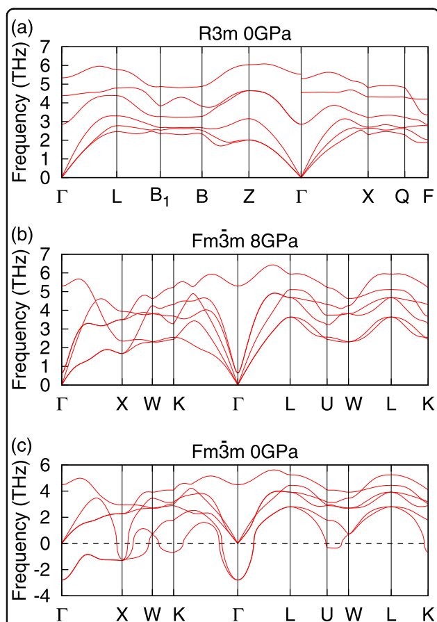
Fig. 2 Phonon dispersions of the different phases of GeSe at selected pressures. The negative values represent imaginary phonon frequencies
