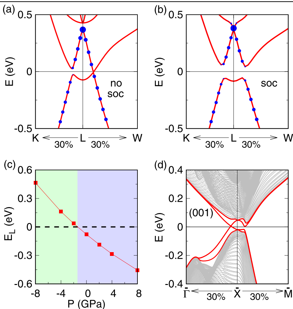
Fig. 5 Band inversion of the rock-salt GeSe phase. Electronic band structures of the Fm\bar{3}m phase at 8 GPa calculated without SOC (a) and with SOC (b). The evolution of band gap at the high symmetry point, L, from DFT calculations with SOC (c). A negative gap represents that the bands are in an inverse order. The (001) surface band structure around \bar{X} was calculated using the tight-binding method (d). The Fermi level is located at 0 eV. The size of the blue dots in panels (a) and (b) is proportional to the weight of the Ge 4s orbitals. The red curves in panel (d) represent the surface bands
